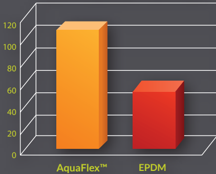
Tensile Strength (LBS) - ASTM D6693
