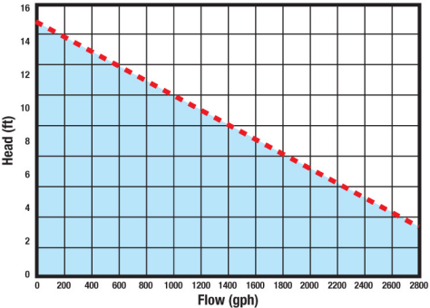
PWM2600 Pump Curve
