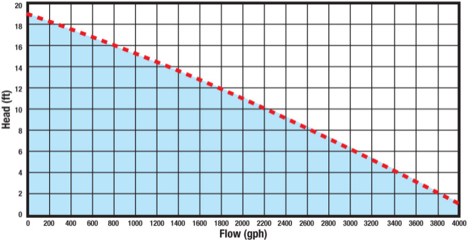
PWM3900 Pump Curve
