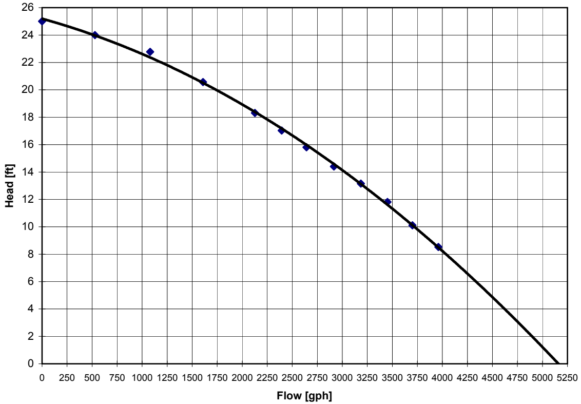
PW4500 Pump Curve (Reduced head)
