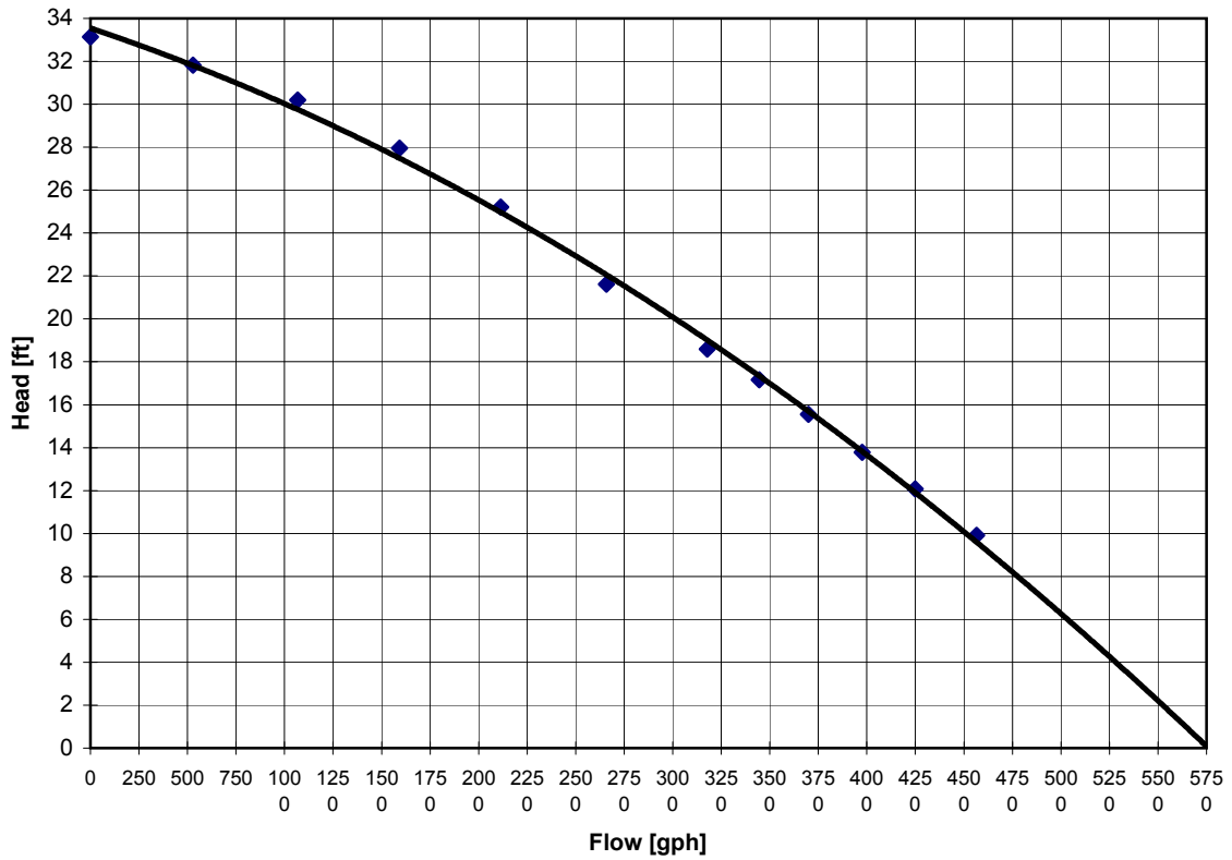
PW5500 Pump Curve (Reduced head)
