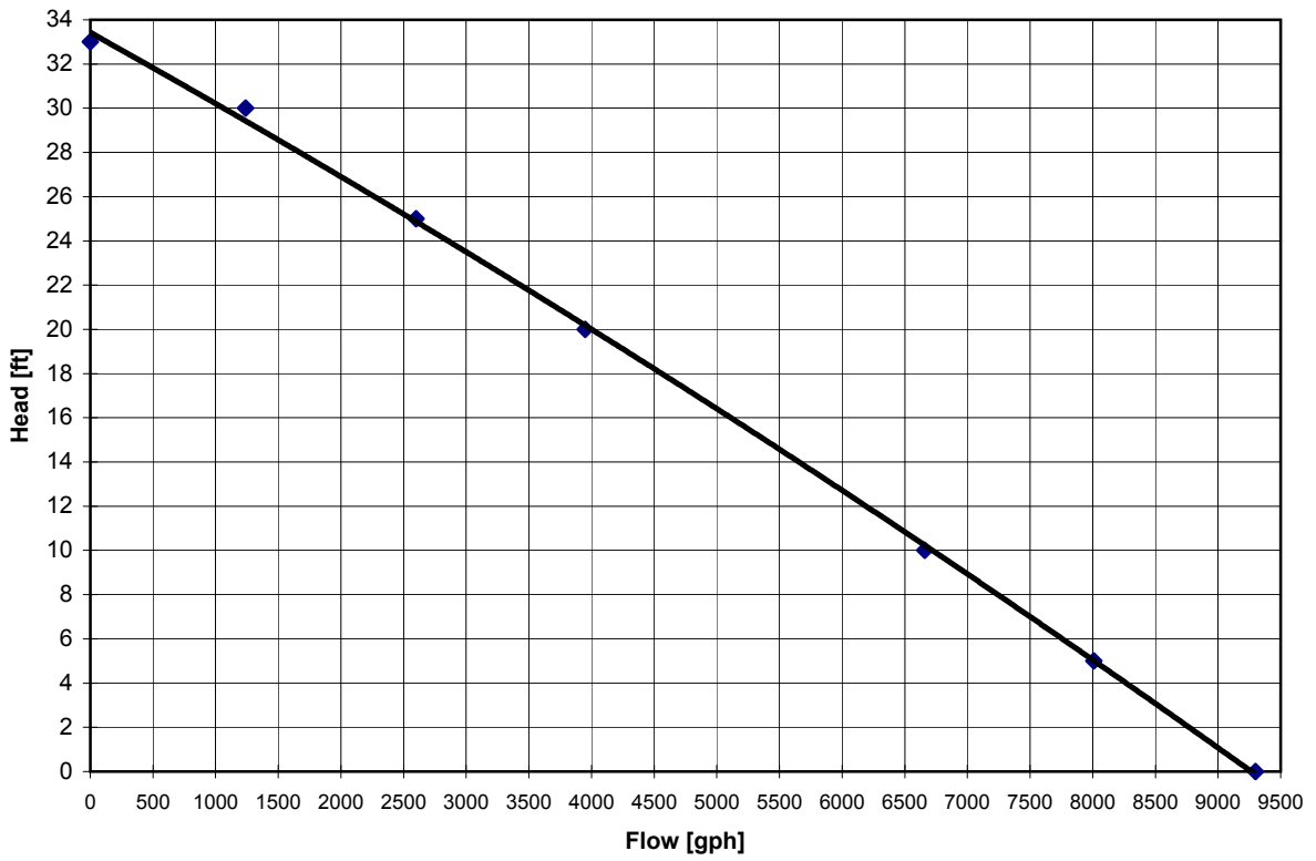
T7500 Pump Curve Torpedo
